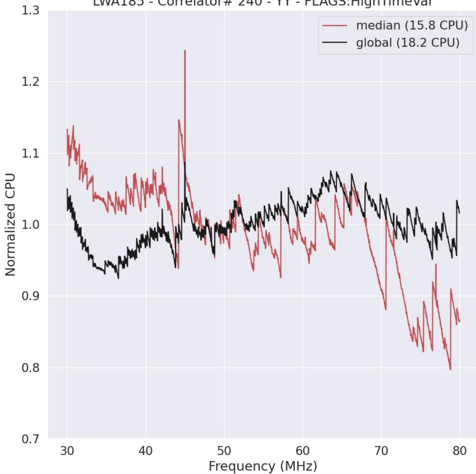
LWA185 - Correlator# 240 - YY - FLAGS:HighTimeVar
