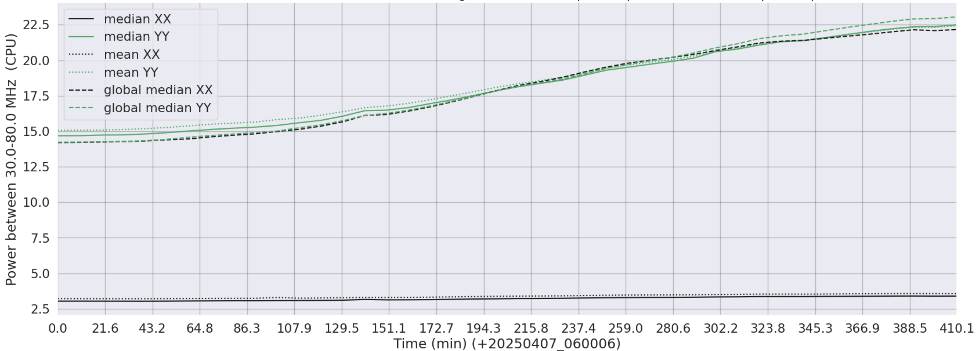
LWA129 - Correlator# 180 - XX FLAGS:HighTimeVar+BadSpecShape - YY FLAGS:BadSpecShape
