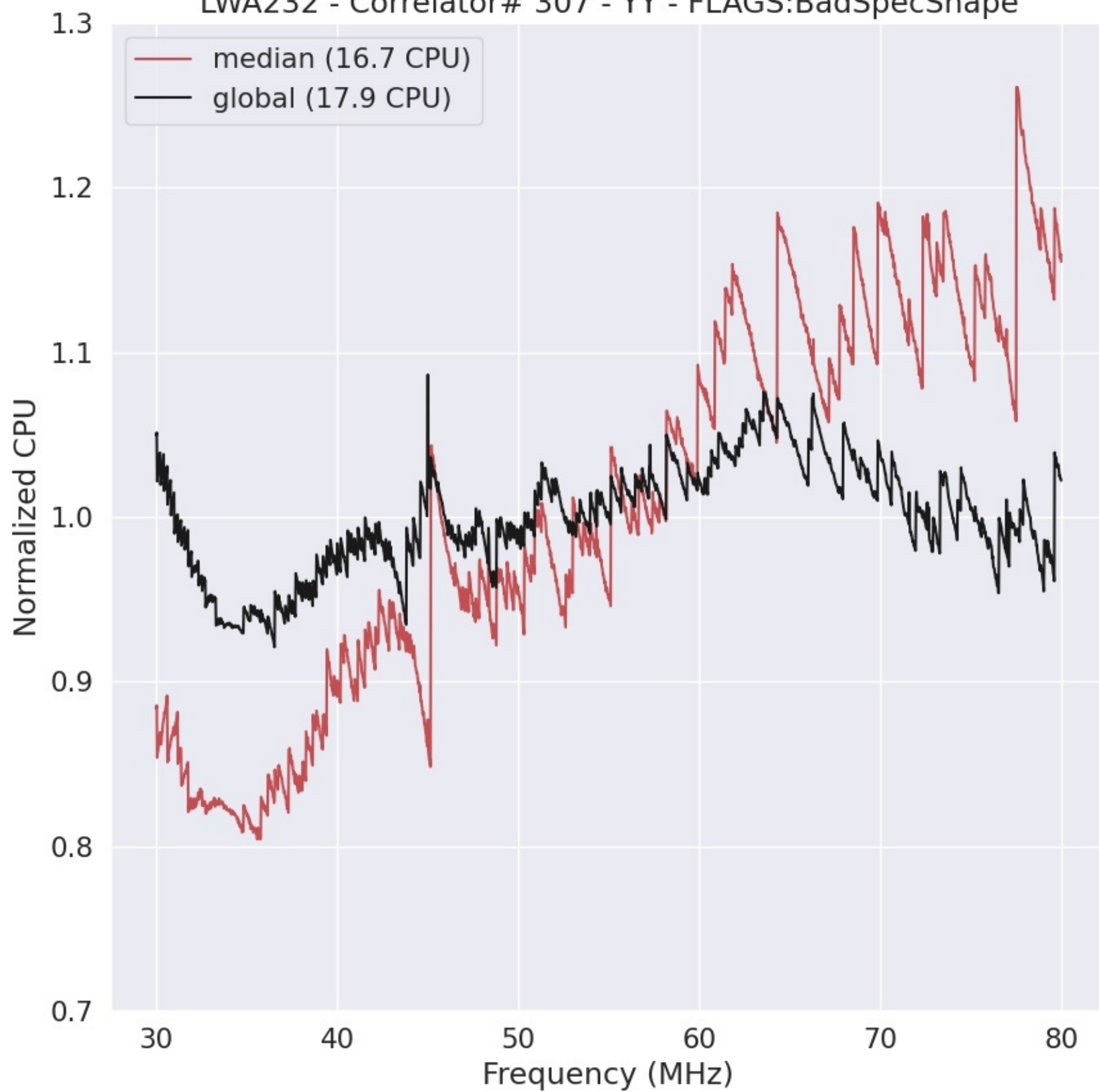
LWA232 - Correlator# 307 - YY - FLAGS:BadSpecShape
