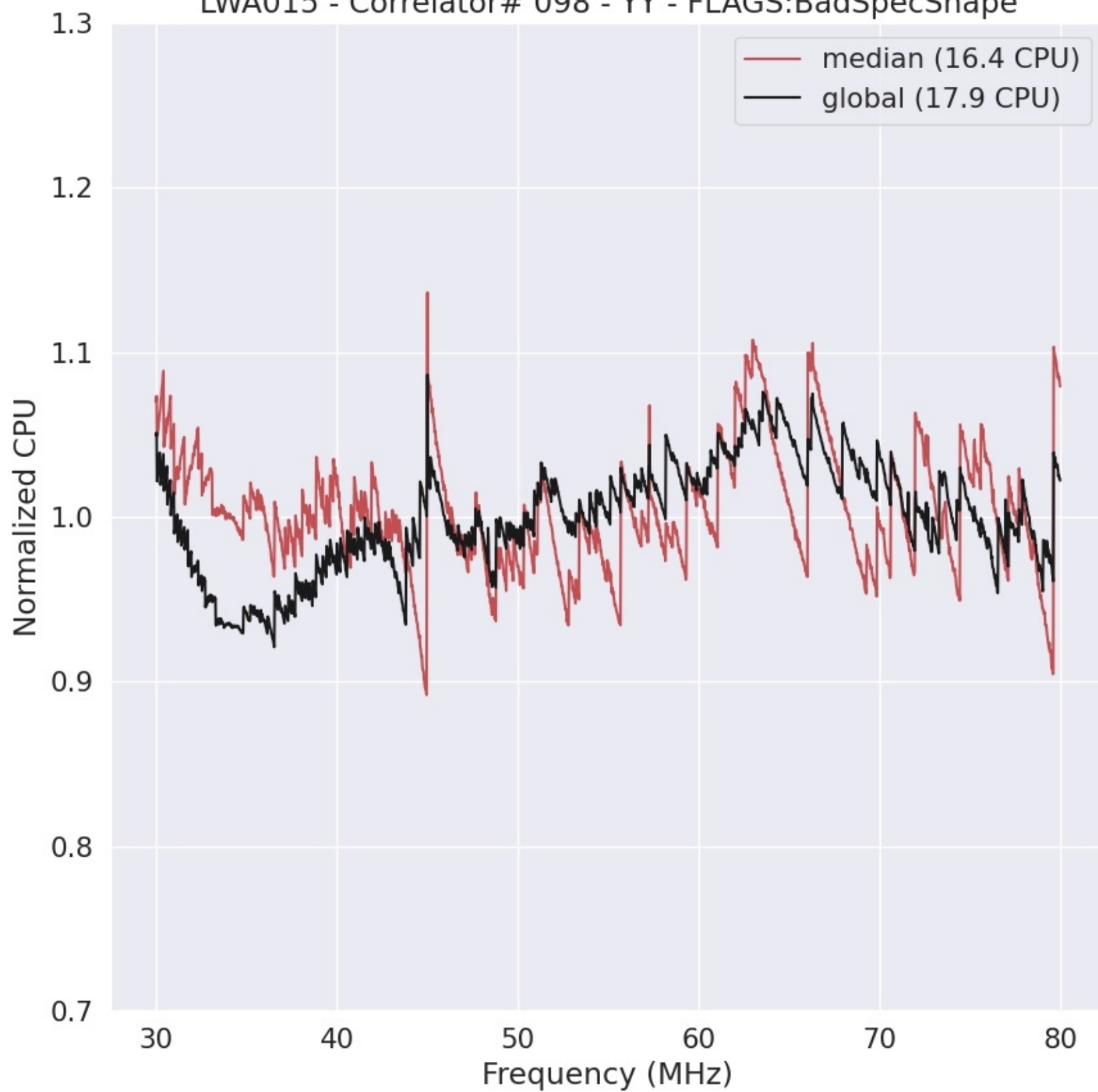
LWA015 - Correlator# 098 - YY - FLAGS:BadSpecShape
