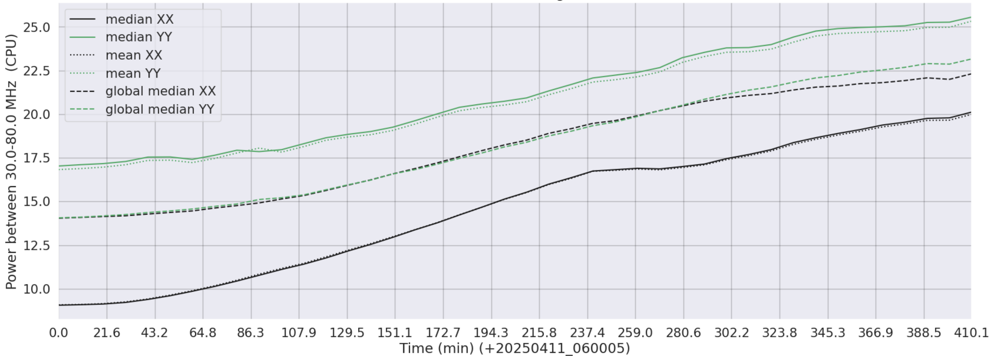
LWA308 - Correlator# 015 - XX FLAGS:HighTimeVar - YY FLAGS:Good
