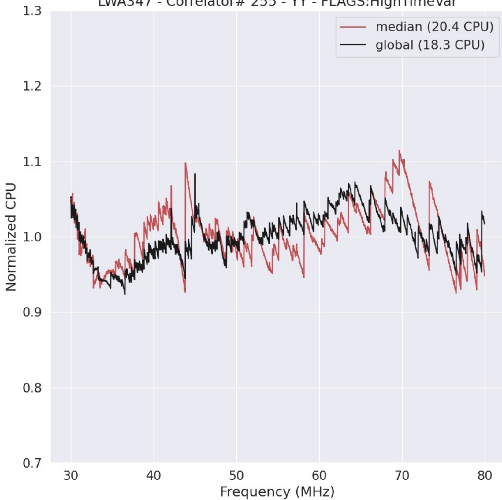
LWA347 - Correlator# 255 - YY - FLAGS:HighTimeVar
