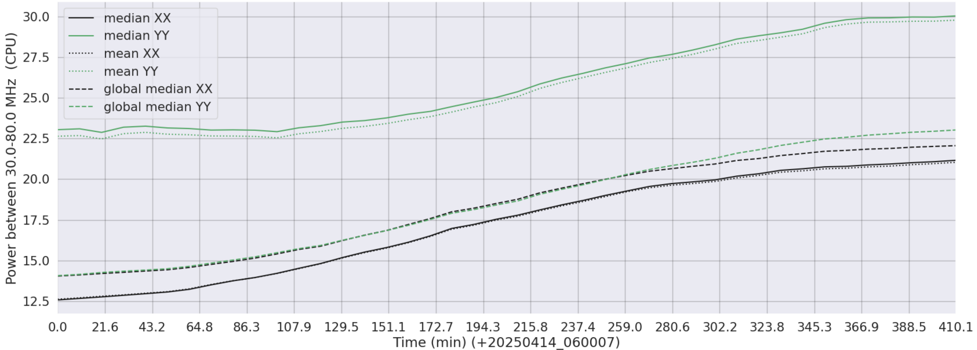
LWA303 - Correlator# 051 - XX FLAGS:Good - YY FLAGS:HighTimeVar
