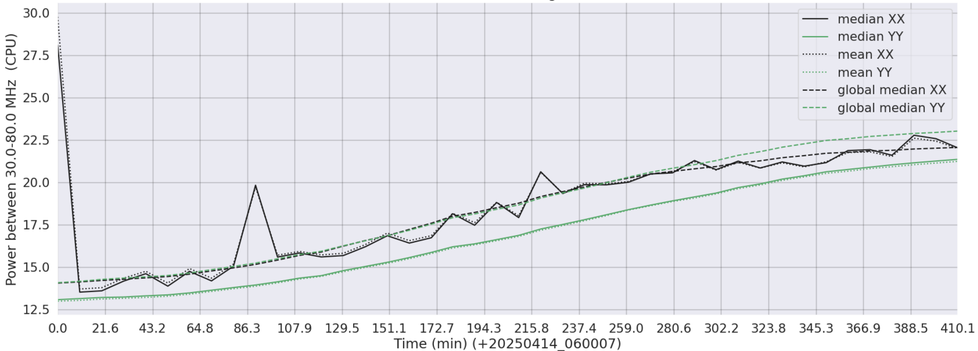
LWA071 - Correlator# 084 - XX FLAGS:HighTimeVar - YY FLAGS:Good
