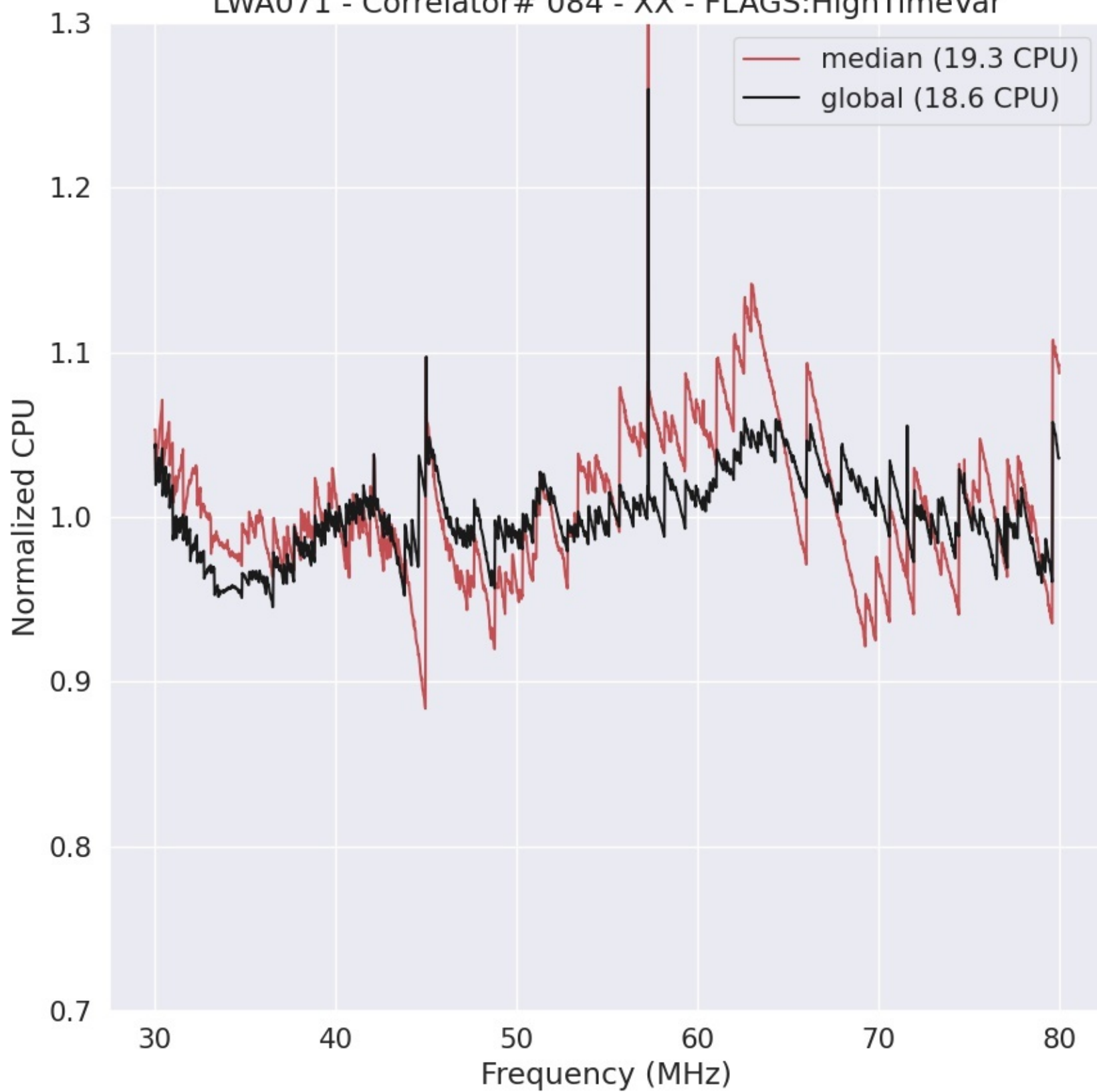
LWA071 - Correlator# 084 - XX - FLAGS:HighTimeVar
