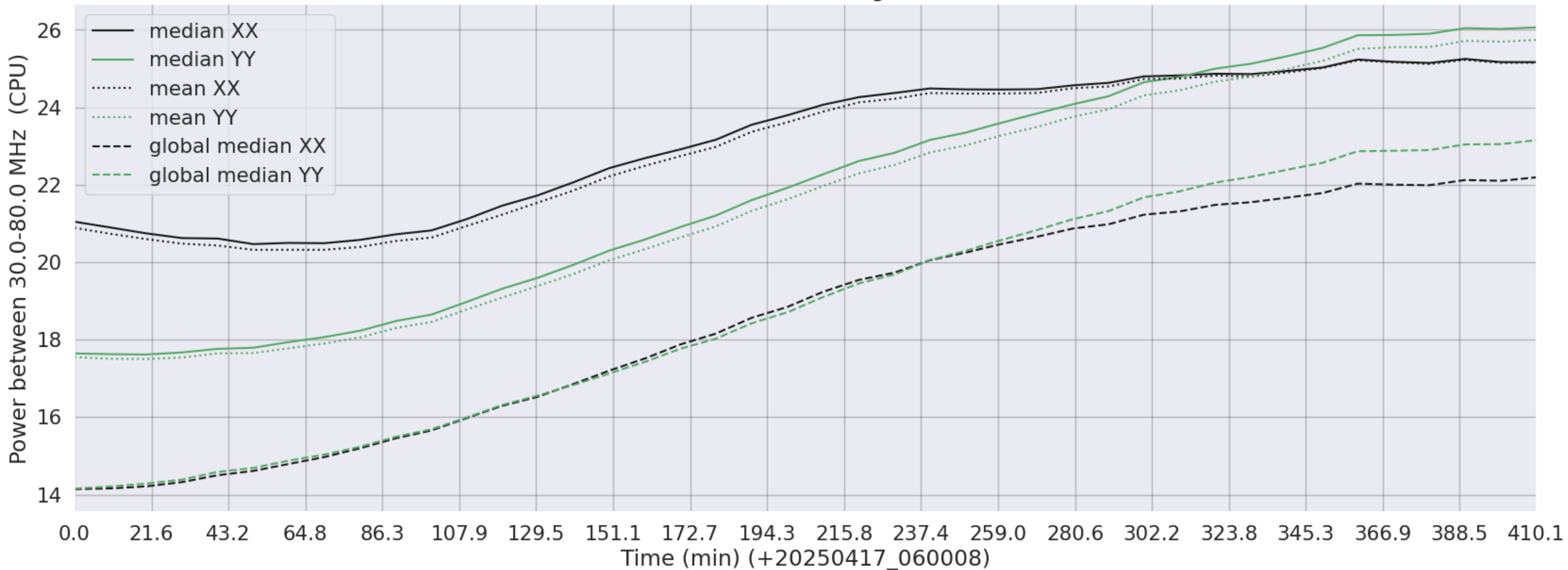
LWA313 - Correlator# 018 - XX FLAGS:HighTimeVar - YY FLAGS:Good
