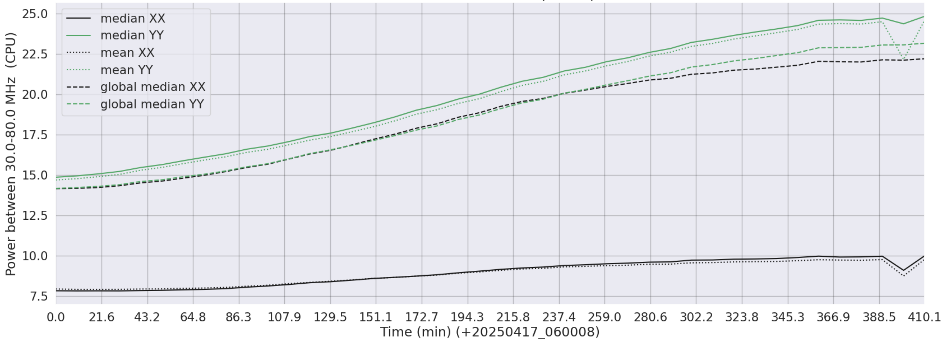
LWA317 - Correlator# 052 - XX FLAGS:BadSpecShape - YY FLAGS:Good
