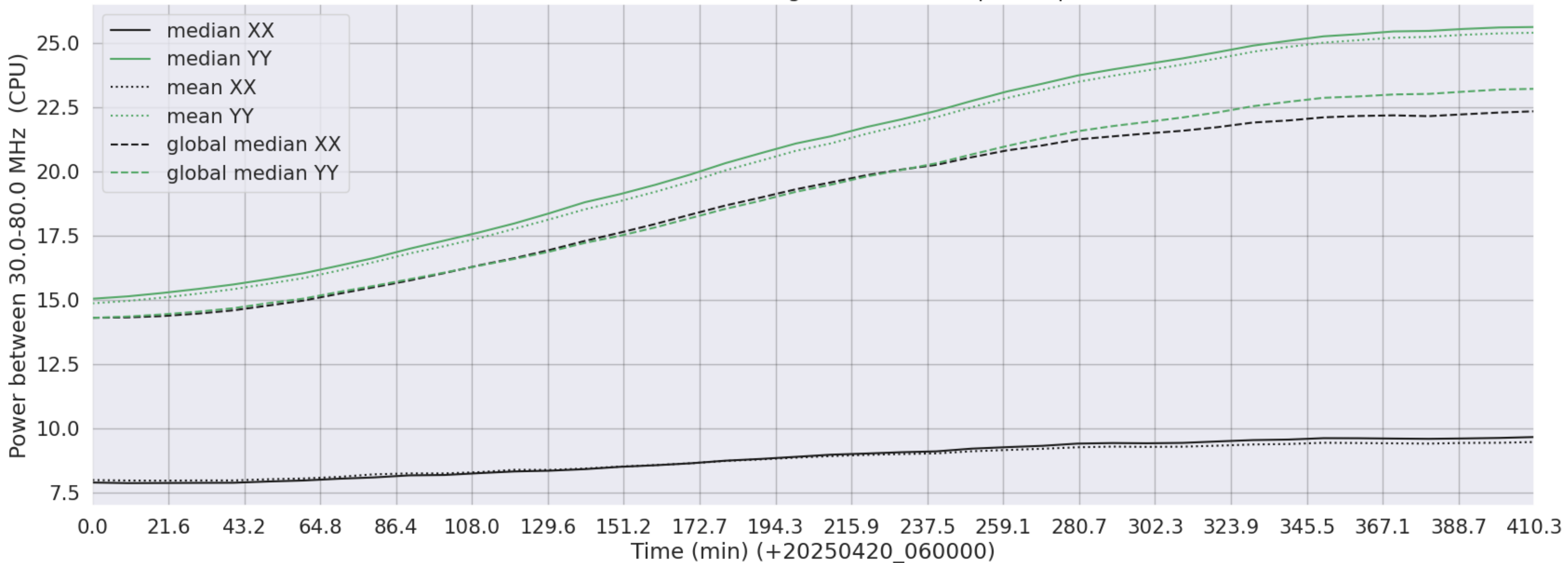
LWA317 - Correlator# 052 - XX FLAGS:HighTimeVar+BadSpecShape - YY FLAGS:Good
