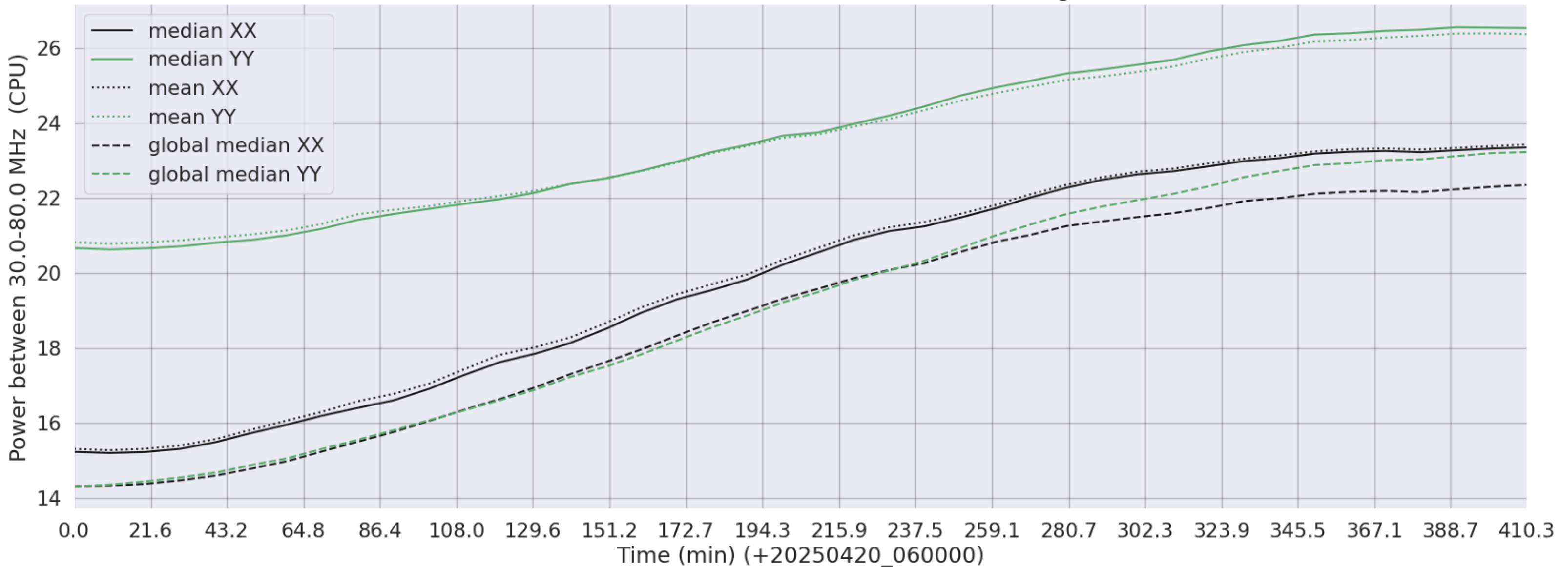
LWA358 - Correlator# 159 - XX FLAGS:Good - YY FLAGS:HighTimeVar
