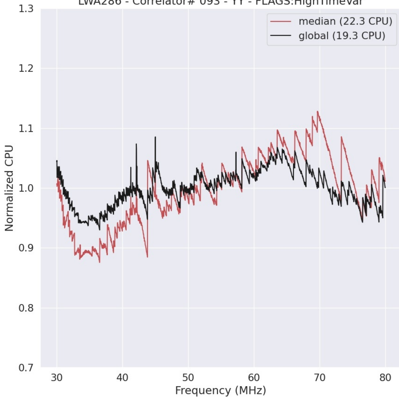
LWA286 - Correlator# 093 - YY - FLAGS:HighTimeVar
