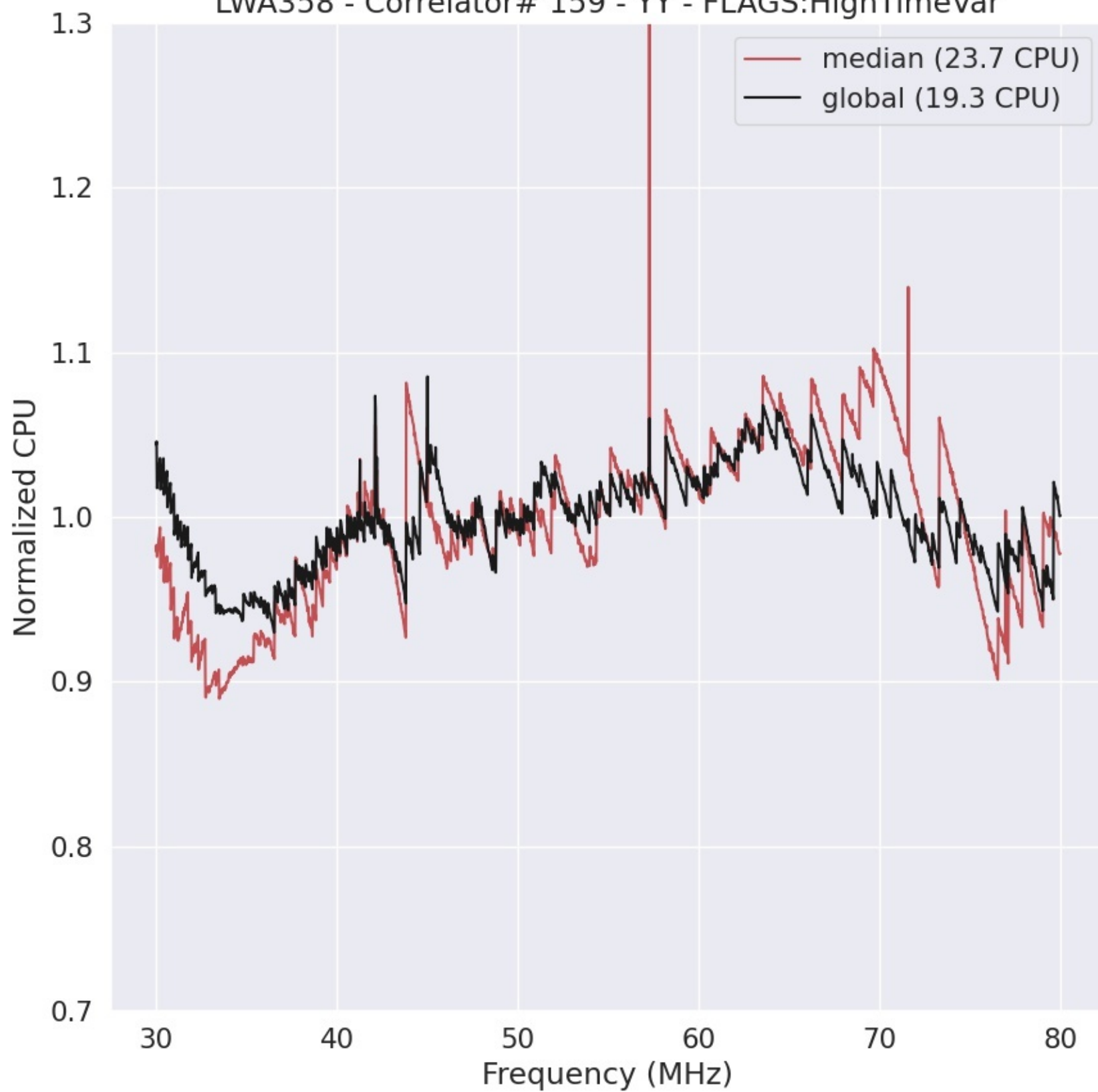
LWA358 - Correlator# 159 - YY - FLAGS:HighTimeVar
