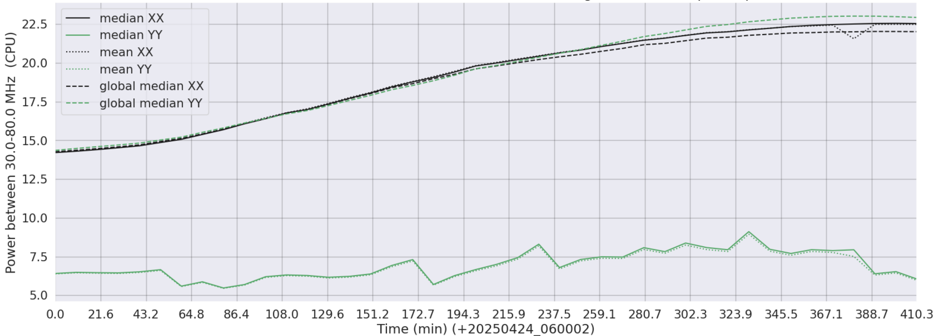
LWA185 - Correlator# 240 - XX FLAGS:Good - YY FLAGS:HighTimeVar+BadSpecShape
