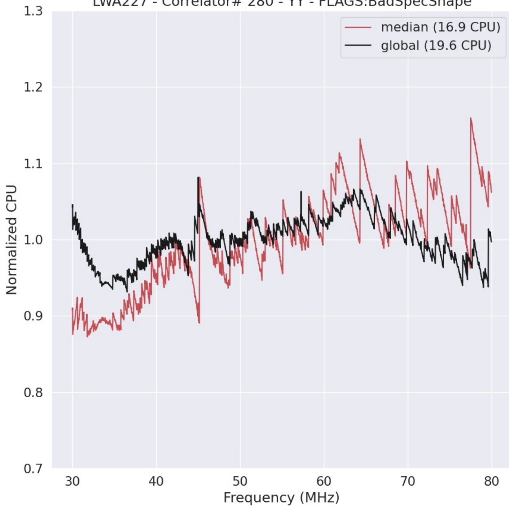
LWA227 - Correlator# 280 - YY - FLAGS:BadSpecShape
