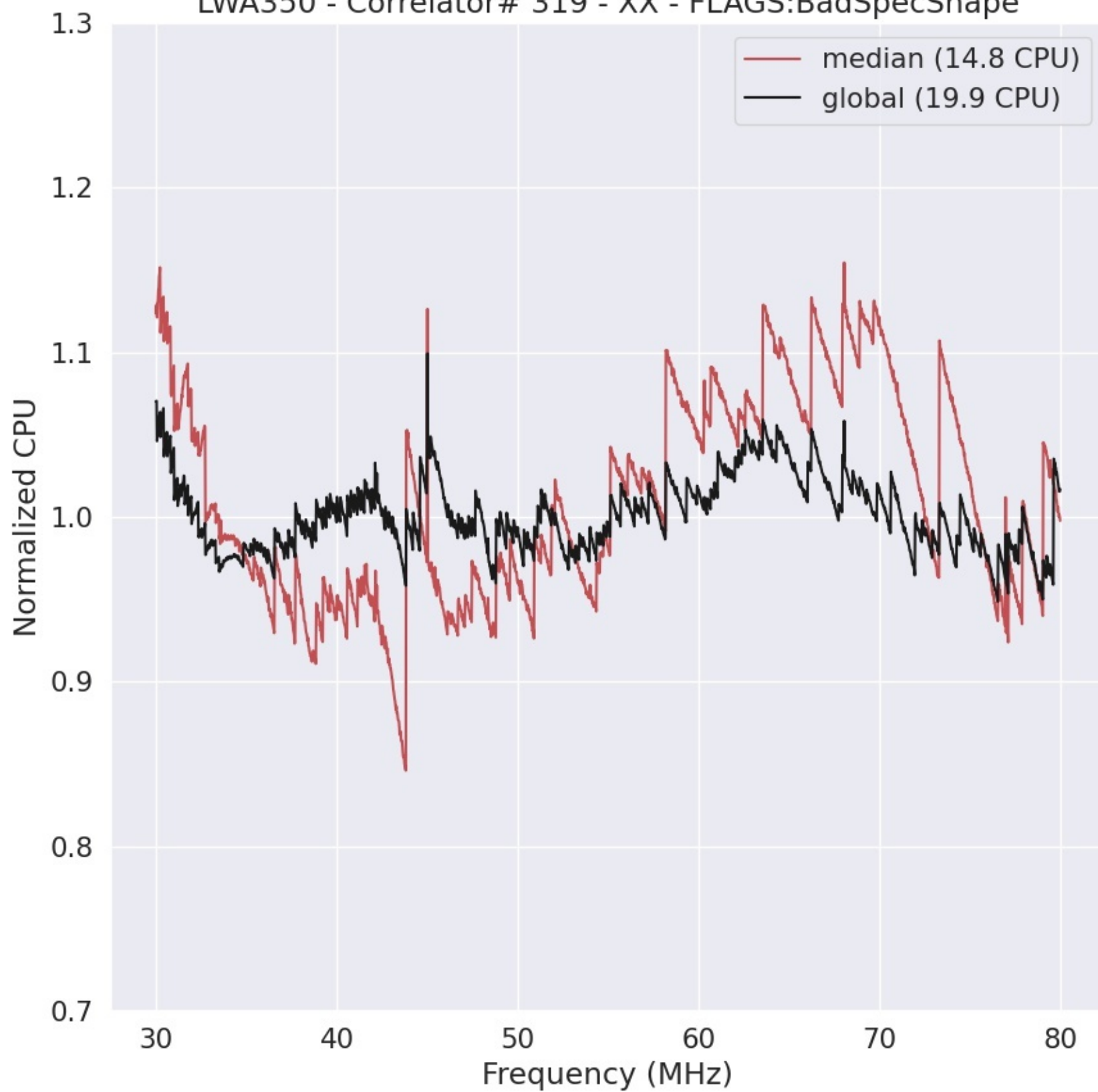
LWA350 - Correlator# 319 - XX - FLAGS:BadSpecShape
