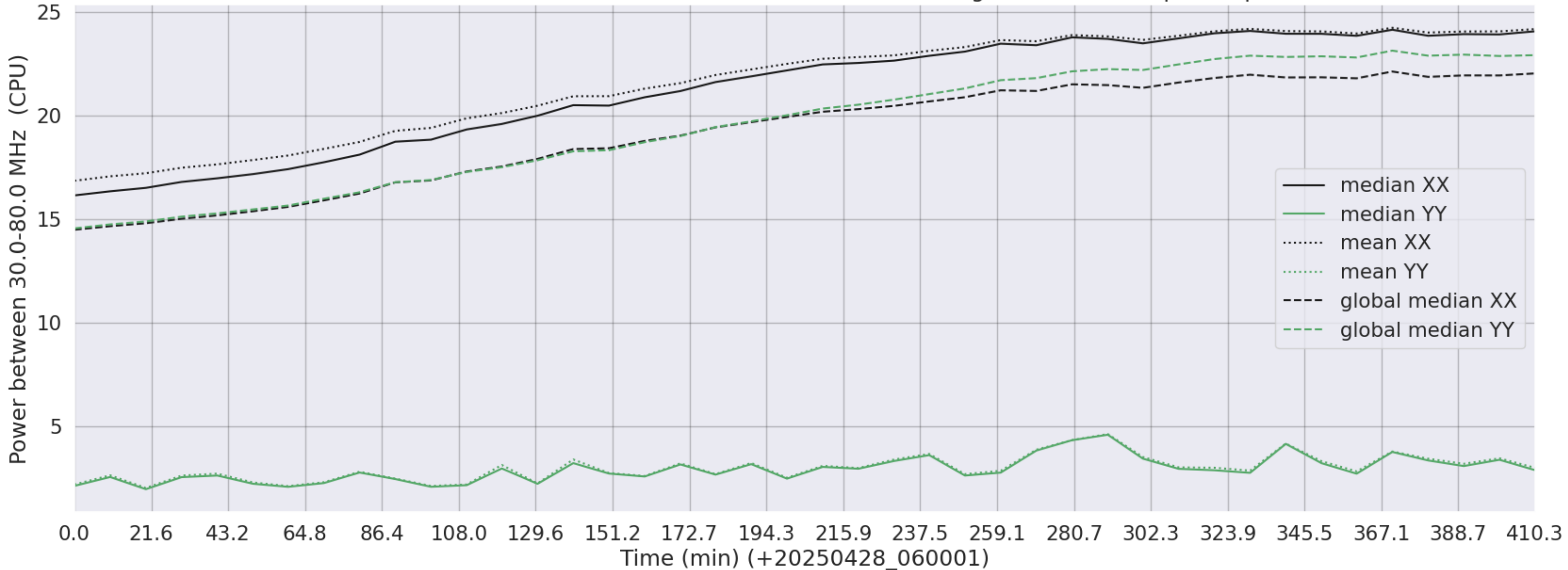
LWA227 - Correlator# 280 - XX FLAGS:Good - YY FLAGS:HighTimeVar+BadSpecShape
