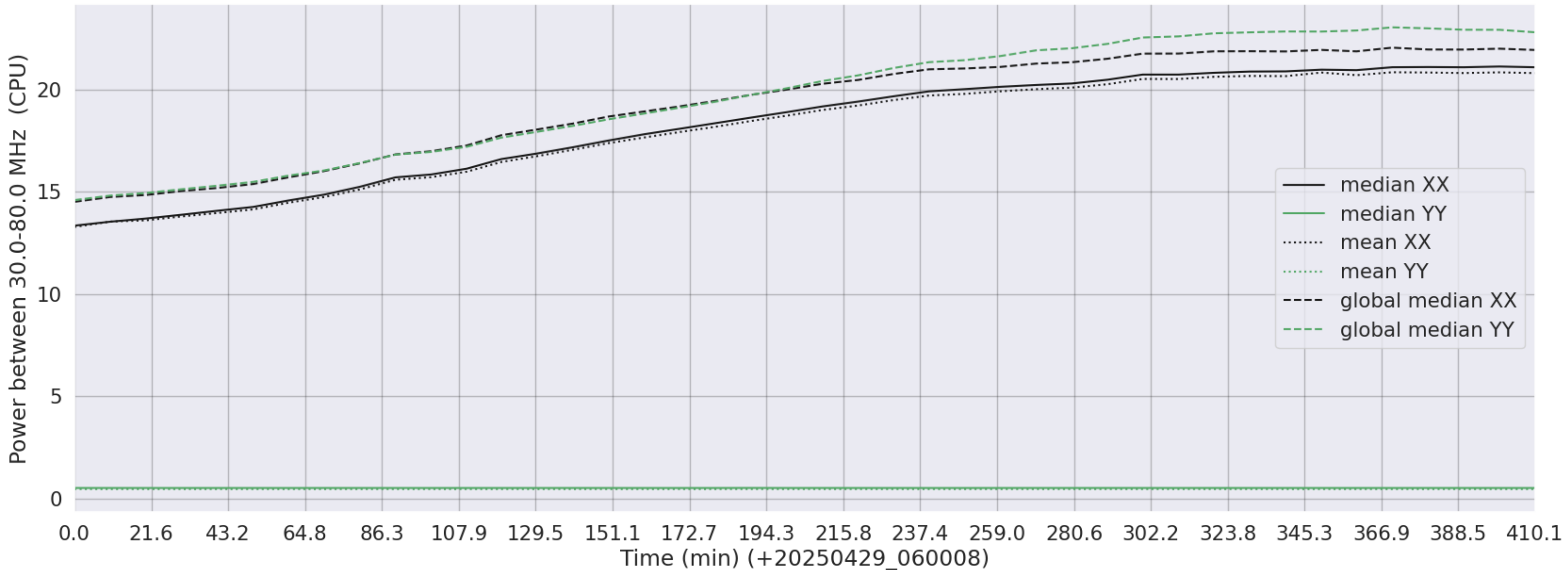
LWA127 - Correlator# 225 - XX FLAGS:Good - YY FLAGS:LowPower
