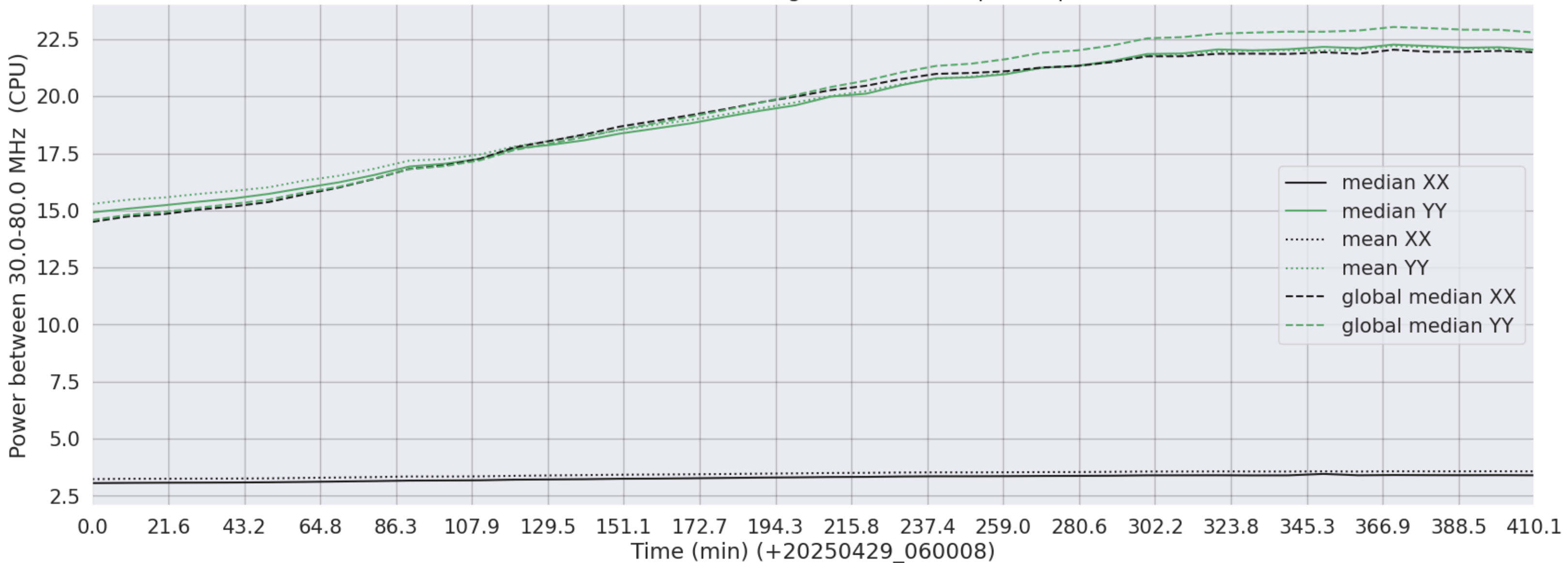
LWA129 - Correlator# 180 - XX FLAGS:HighTimeVar+BadSpecShape - YY FLAGS:Good
