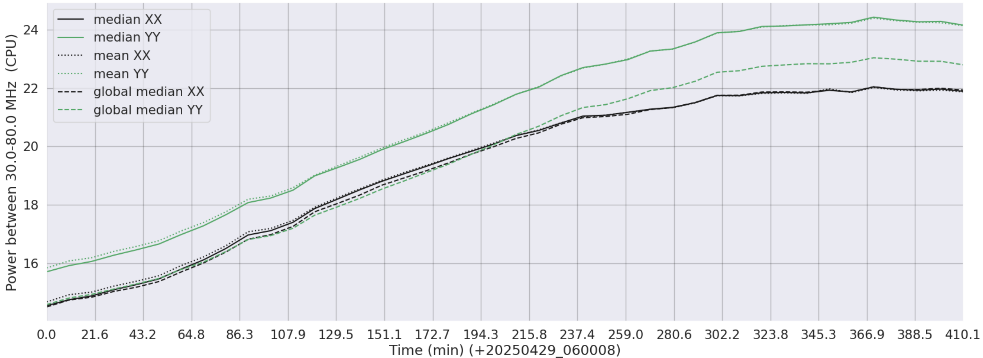
LWA234 - Correlator# 289 - XX FLAGS:Good - YY FLAGS:Good
