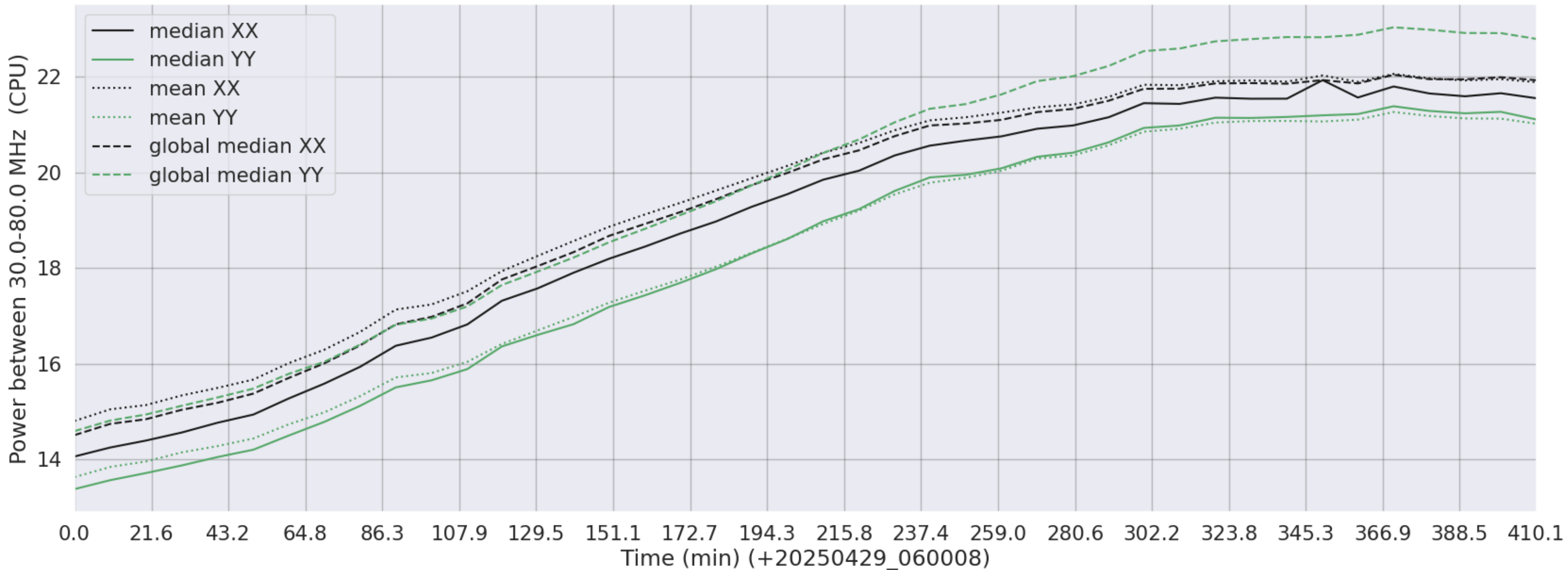
LWA232 - Correlator# 307 - XX FLAGS:Good - YY FLAGS:Good
