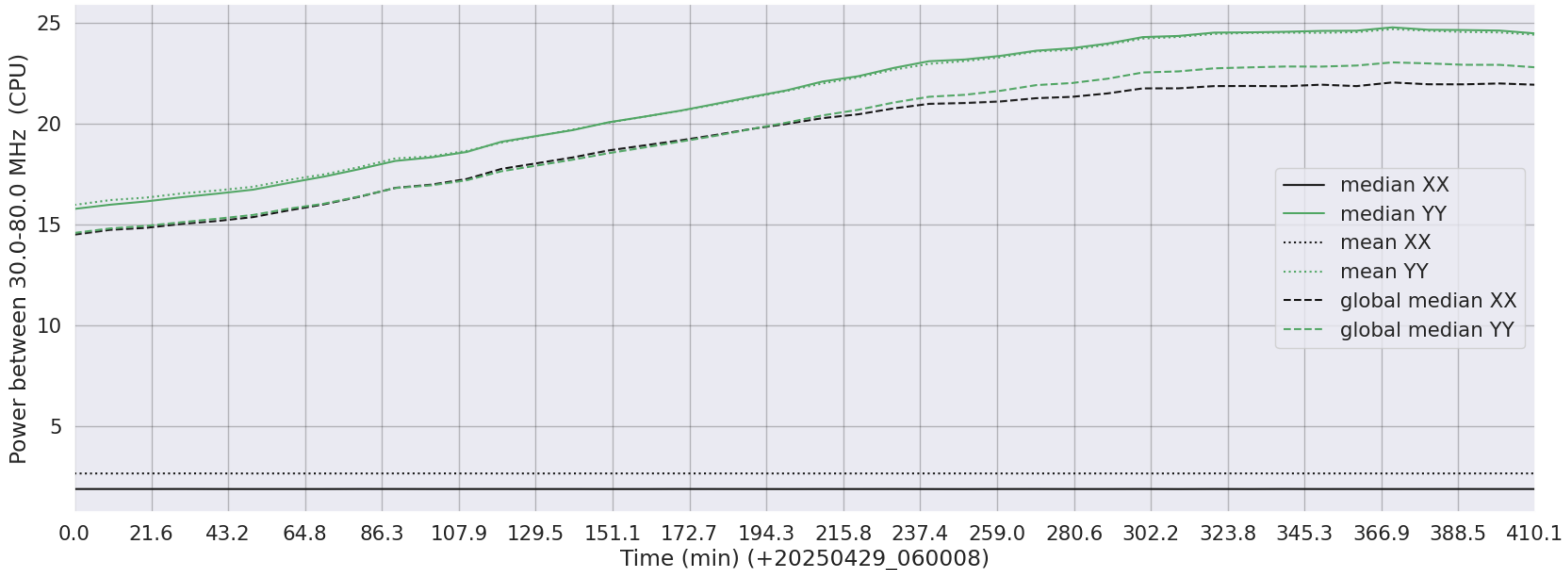
LWA203 - Correlator# 295 - XX FLAGS:LowPower - YY FLAGS:Good
