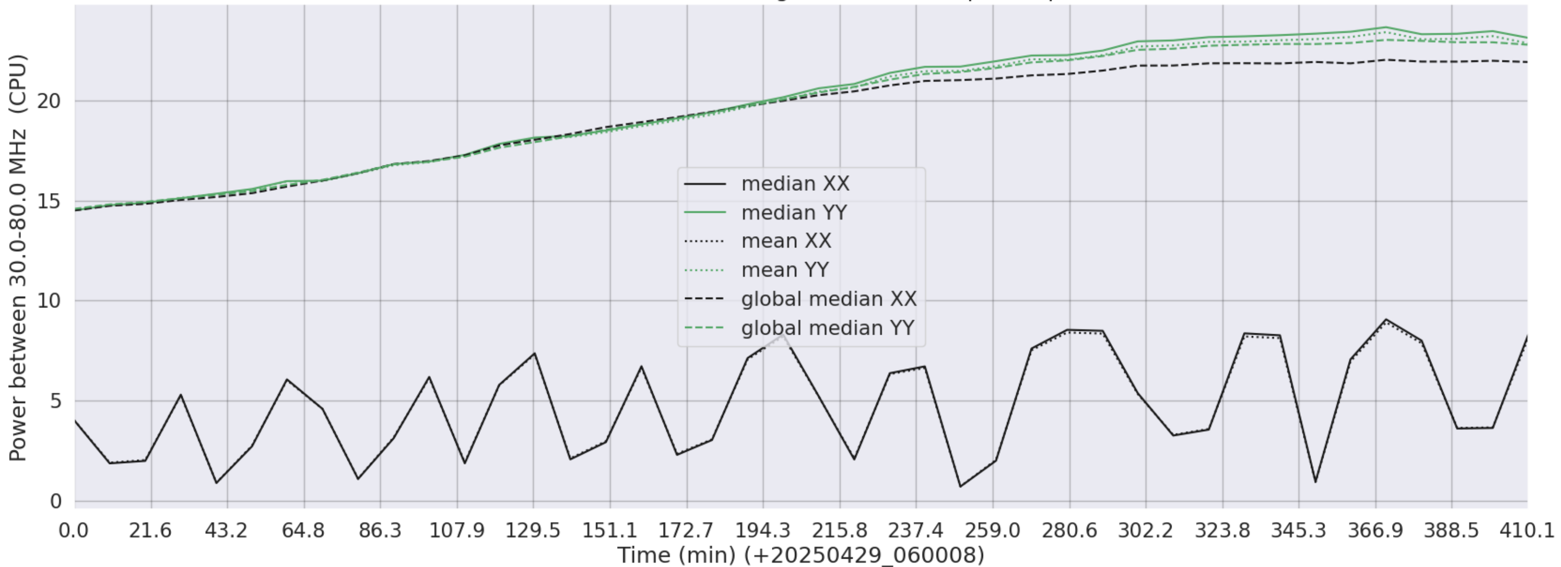
LWA124 - Correlator# 224 - XX FLAGS:HighTimeVar+BadSpecShape - YY FLAGS:Good
