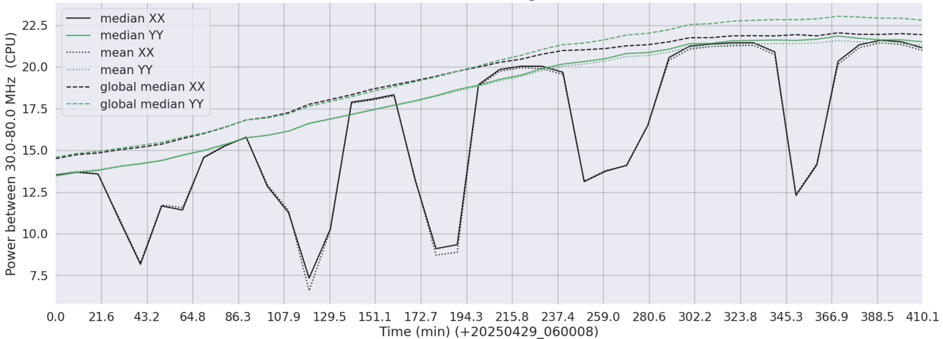
LWA249 - Correlator# 342 - XX FLAGS:HighTimeVar - YY FLAGS:Good
