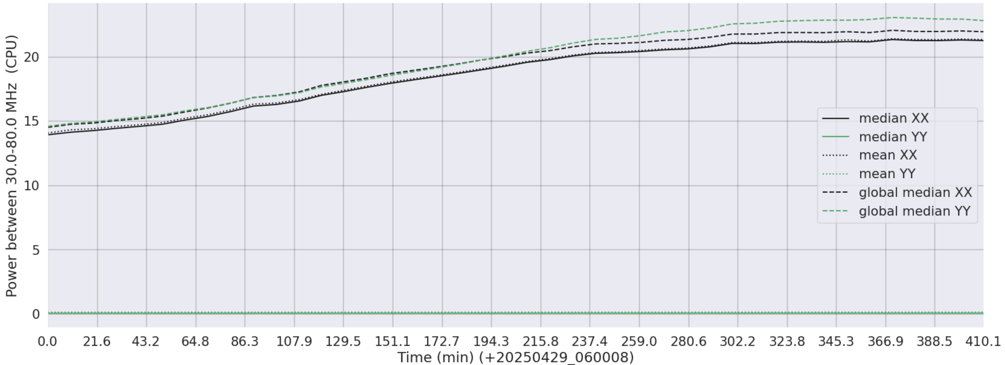
LWA235 - Correlator# 309 - XX FLAGS:Good - YY FLAGS:LowPower
