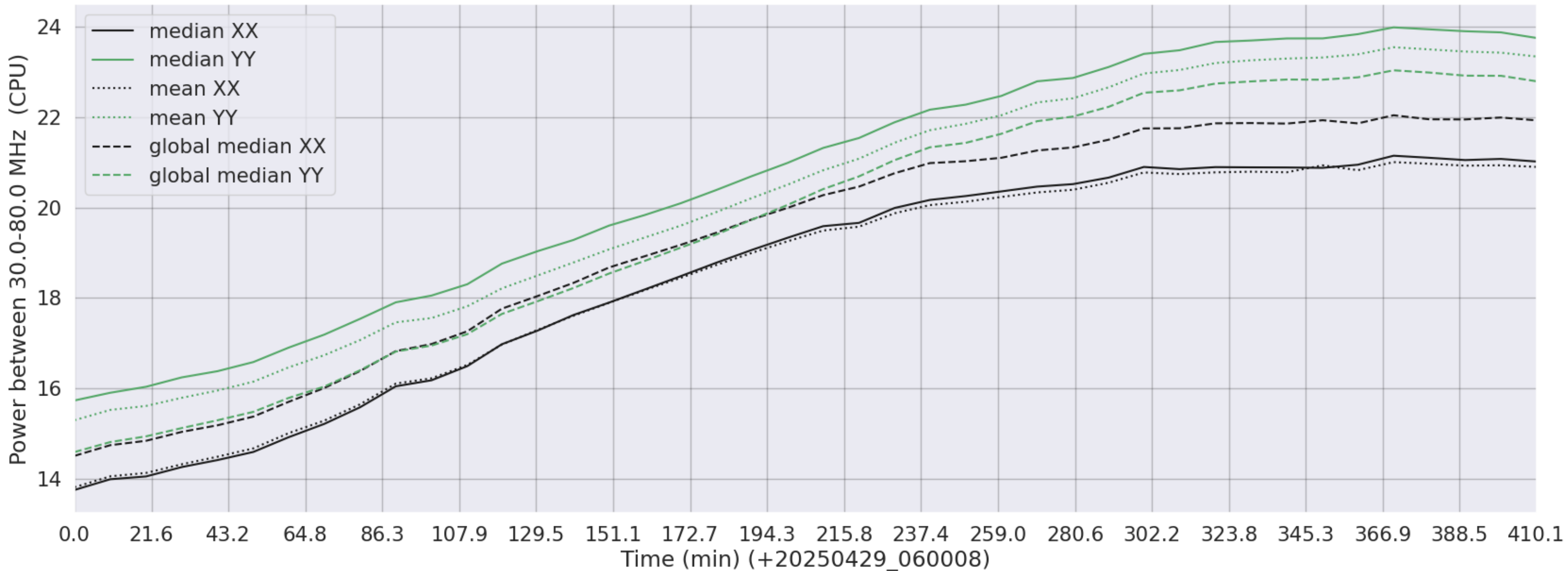
LWA138 - Correlator# 261 - XX FLAGS:Good - YY FLAGS:Good
