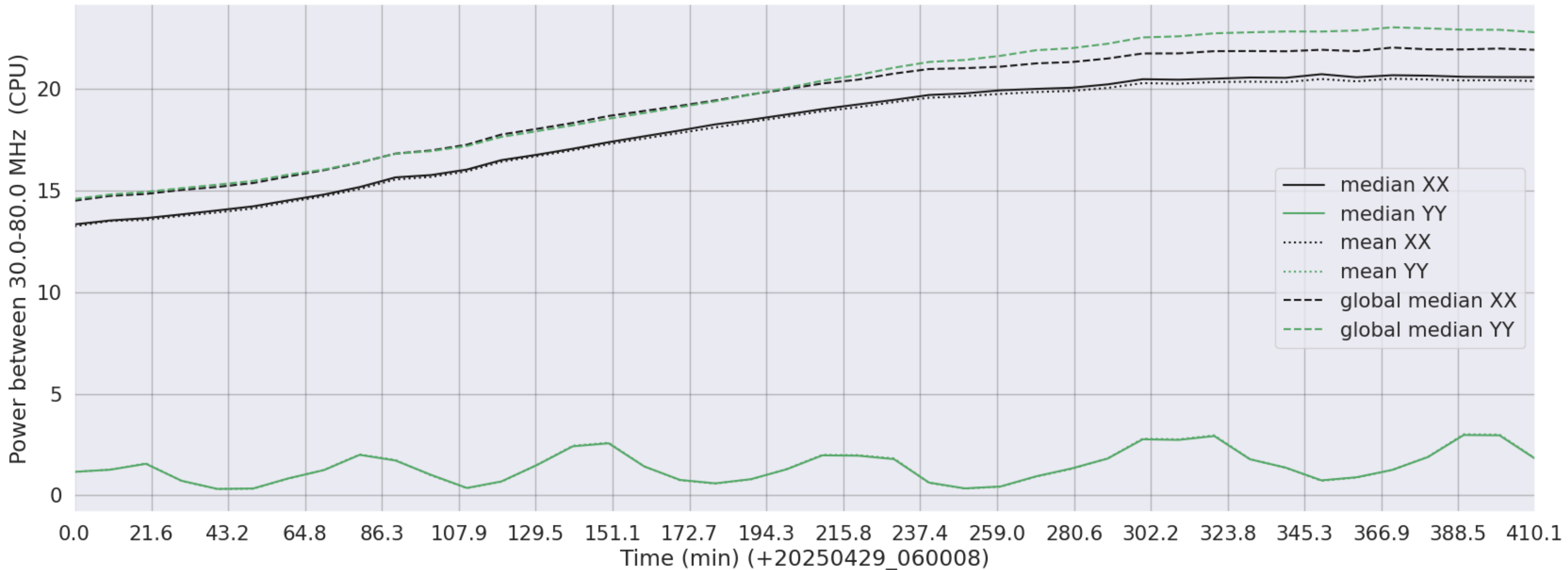
LWA189 - Correlator# 245 - XX FLAGS:Good - YY FLAGS:LowPower
