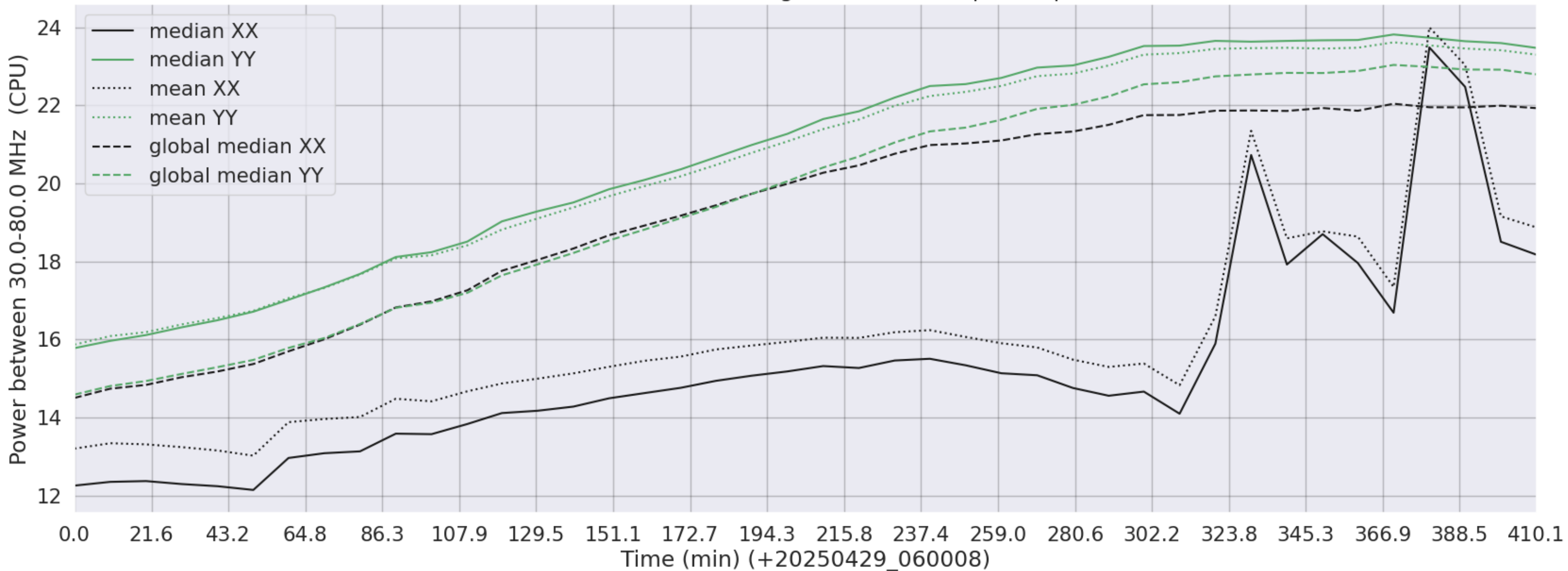
LWA131 - Correlator# 182 - XX FLAGS:HighTimeVar+BadSpecShape - YY FLAGS:Good
