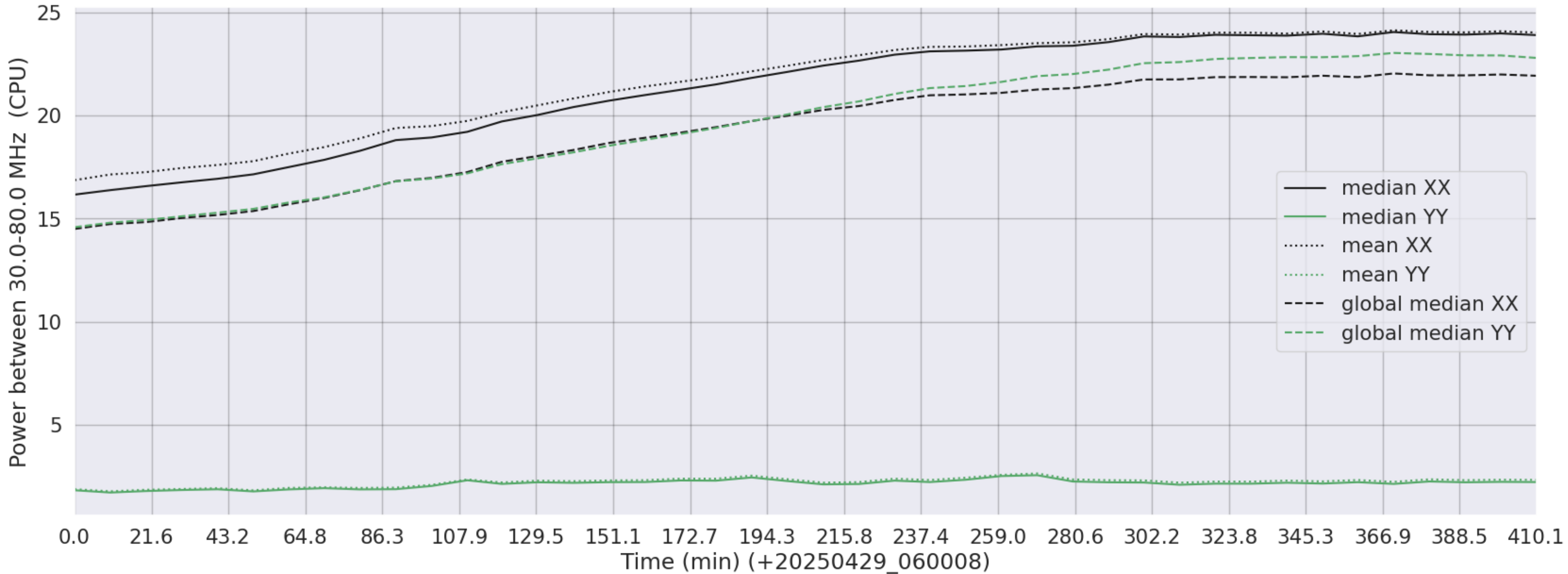
LWA227 - Correlator# 280 - XX FLAGS:Good - YY FLAGS:LowPower
