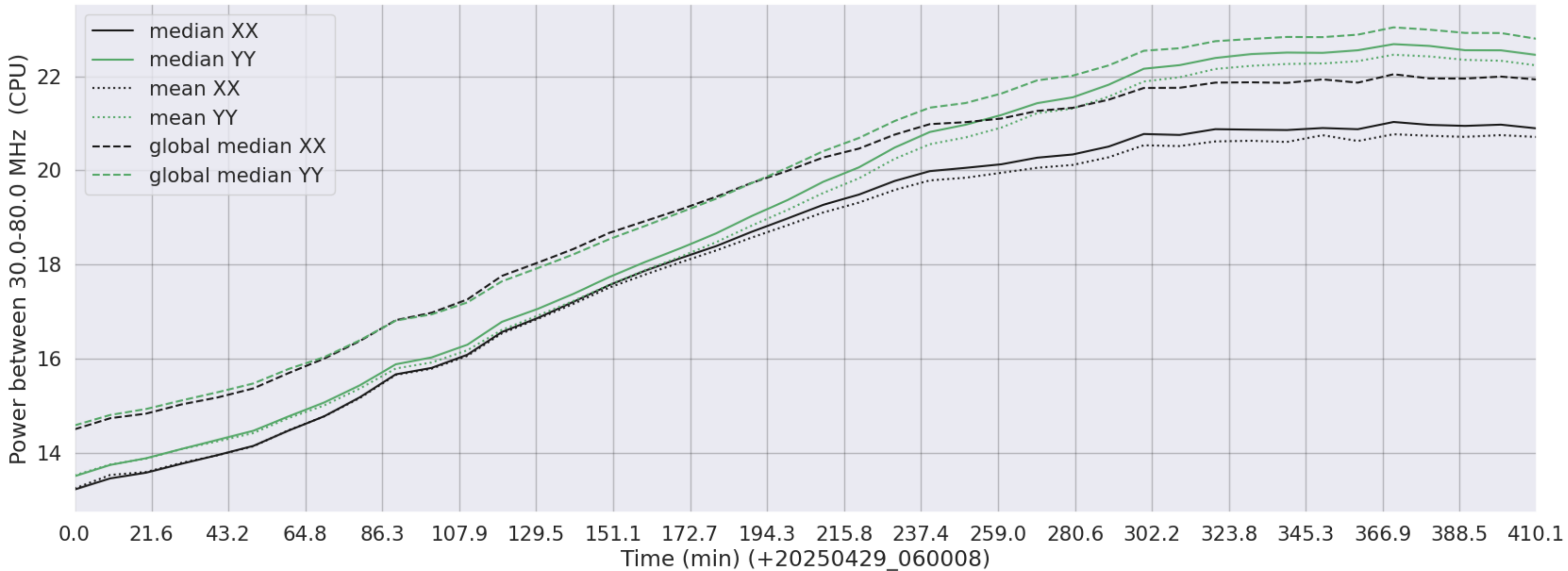
LWA187 - Correlator# 242 - XX FLAGS:Good - YY FLAGS:Good
