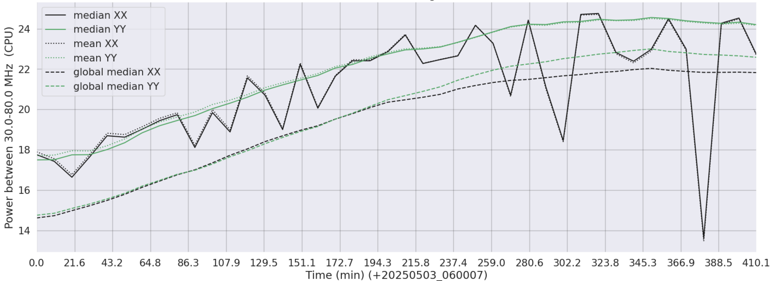
LWA334 - Correlator# 156 - XX FLAGS:HighTimeVar - YY FLAGS:Good
