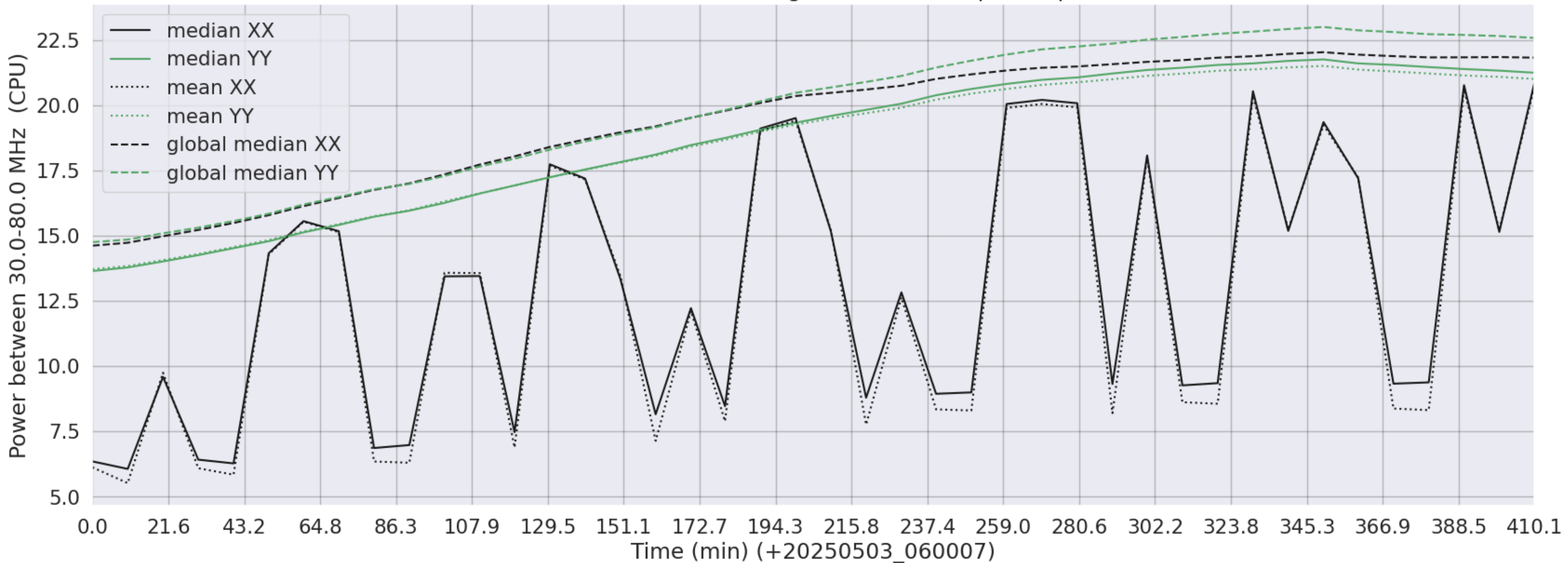
LWA249 - Correlator# 342 - XX FLAGS:HighTimeVar+BadSpecShape - YY FLAGS:Good
