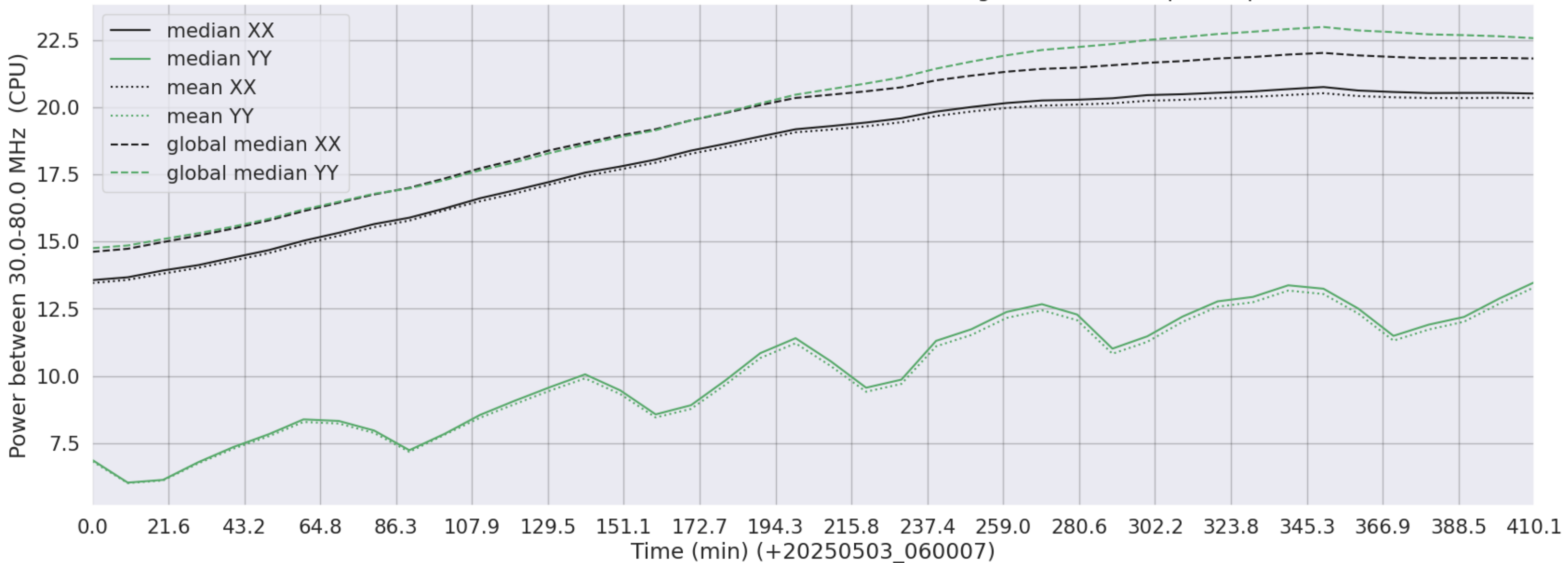
LWA189 - Correlator# 245 - XX FLAGS:Good - YY FLAGS:HighTimeVar+BadSpecShape
