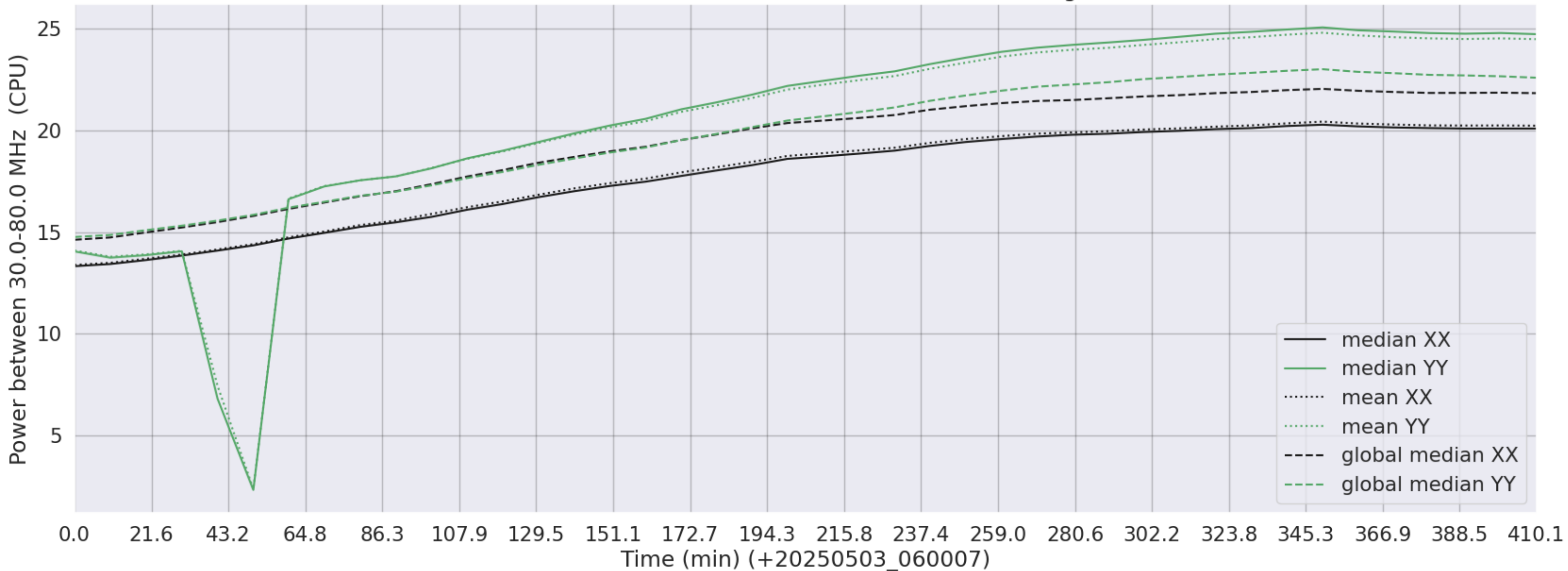
LWA244 - Correlator# 338 - XX FLAGS:Good - YY FLAGS:HighTimeVar
